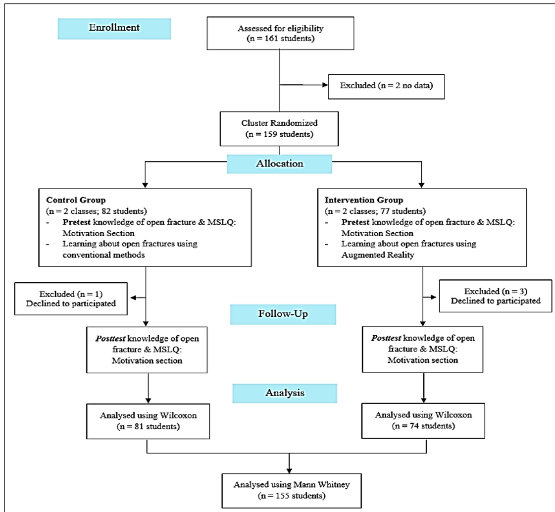
Figure 1. Research Flowchart
